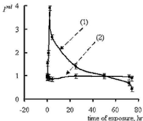
Fig. 1 Bioluminescent intensity ( I^{rel} ) vs time of exposure ( t , hours) in solutions of ^{241}\text{Am}^{3+} ( C = 2 \cdot 10^{-10} M, A = 6000 Bq/l) (1) and \text{Eu}^{3+} ( C = 2 \cdot 10^{-10} M) (2), from: (Rozhko et al., 2007)
