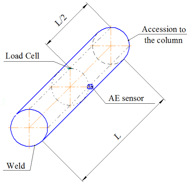
Figure 3. Arrangement of the sensors in the horizontal section of the gas pipeline connected to the column.
