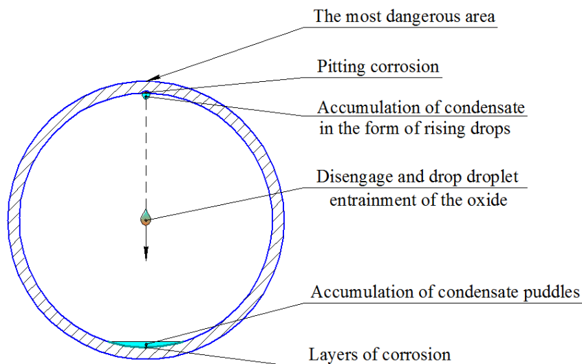
Figure 1. The accumulation of wet condensate in the horizontal section of the pipeline.
