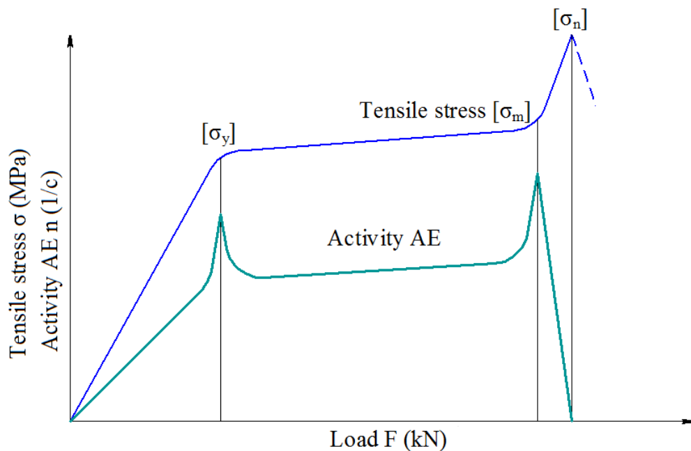
Figure 2. Similarity of the plots of mechanical stress and activity of the AE versus the object load.
