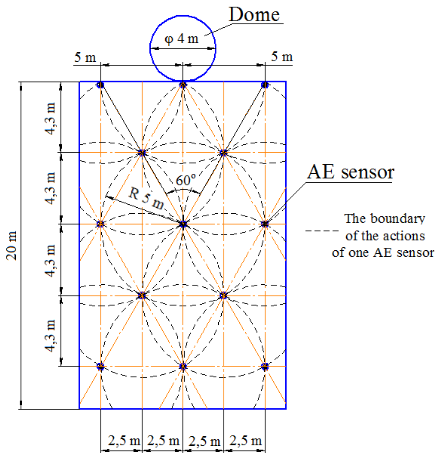
Figure 4. Arrangement of AE sensors to scan the body of the distillation column.
