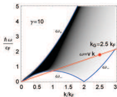
Fig. 3. (Color online) Dynamic structure factor of the 1D Bose gas from [21] for N = 100 . Dimensionless values of S(k, \omega)\epsilon_F/N are shown in shades of gray between 0 (white) and 0.7 (black). The full (blue) lines represent the limiting dispersion relations \omega_{\pm}(k) and the straight (red) line is the line of integration in Eq. (2). Only one point at k = k_G , shown in full (red) circle, contributes to the integral when the perturber is a shallow cosine potential with a reciprocal vector k_G
