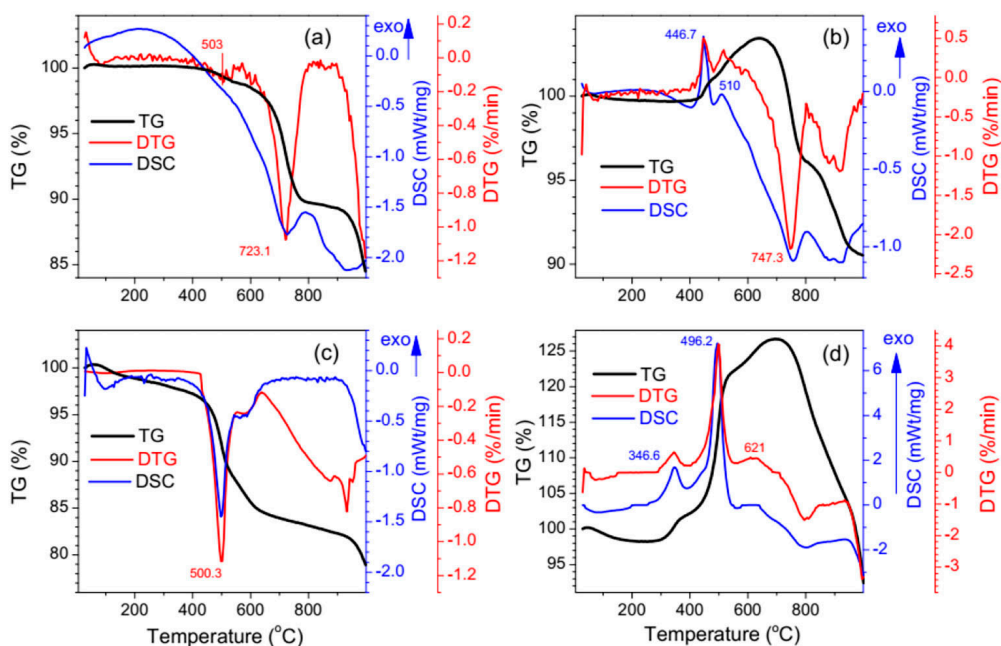
Fig. 5. Thermogravimetric (TG), differential thermogravimetric (DTG), and differential scanning calorimetry (DSC) curves for heating (a),(b) valleriite-containing Kingash sample and (c),(d) synthetic valleriite in (a),(c) inert Ar and (b),(d) air flow
