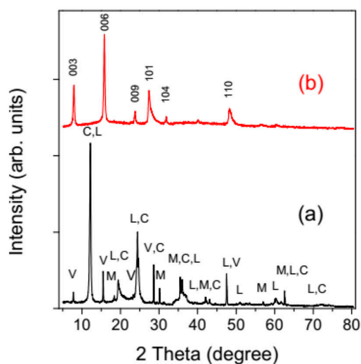
Fig. 1. X-ray diffraction pattern of (a) Kingash valleriite ore in comparison with (b) synthetic valleriite (the main interplanar distances are denoted). Reflections from mineral phases are marked as V belong to valleriite (PDF 01–073–0517), M is magnetite (01–089–3854), L is lizardite-1T high (01–089–6206), C is chrysotile (00–010–0380)
