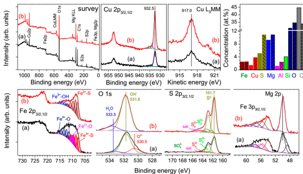
Fig. 4. X-ray photoelectron spectra, and atomic concentrations (histogram) derived from the survey spectrum for (a) Kingash valleriite-containing sample and (b) synthetic valleriite (patterned columns in the concentration histogram)
