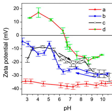
Fig. 6. Zeta potentials of (a) synthetic valleriite nanoflakes and Kingash ore samples measured using (b, c) the flow potential method from the fraction -125 + 75 \mu\text{m} with (b) increasing and (c) decreasing pH and (d) electrophoretic mobility for the fraction -20 \mu\text{m}
