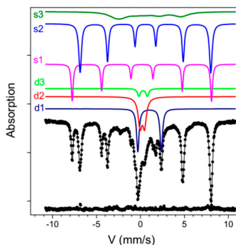
Fig. 3. ^{57}\text{Fe} Mössbauer spectrum (points) of a Kingash rock sample measured at room temperature. The lines are the results of fitting; the difference between experimental spectrum and fitted one also shown was typically within 3 rel.% of the spectrum area. The fit parameters are given in Table 2
