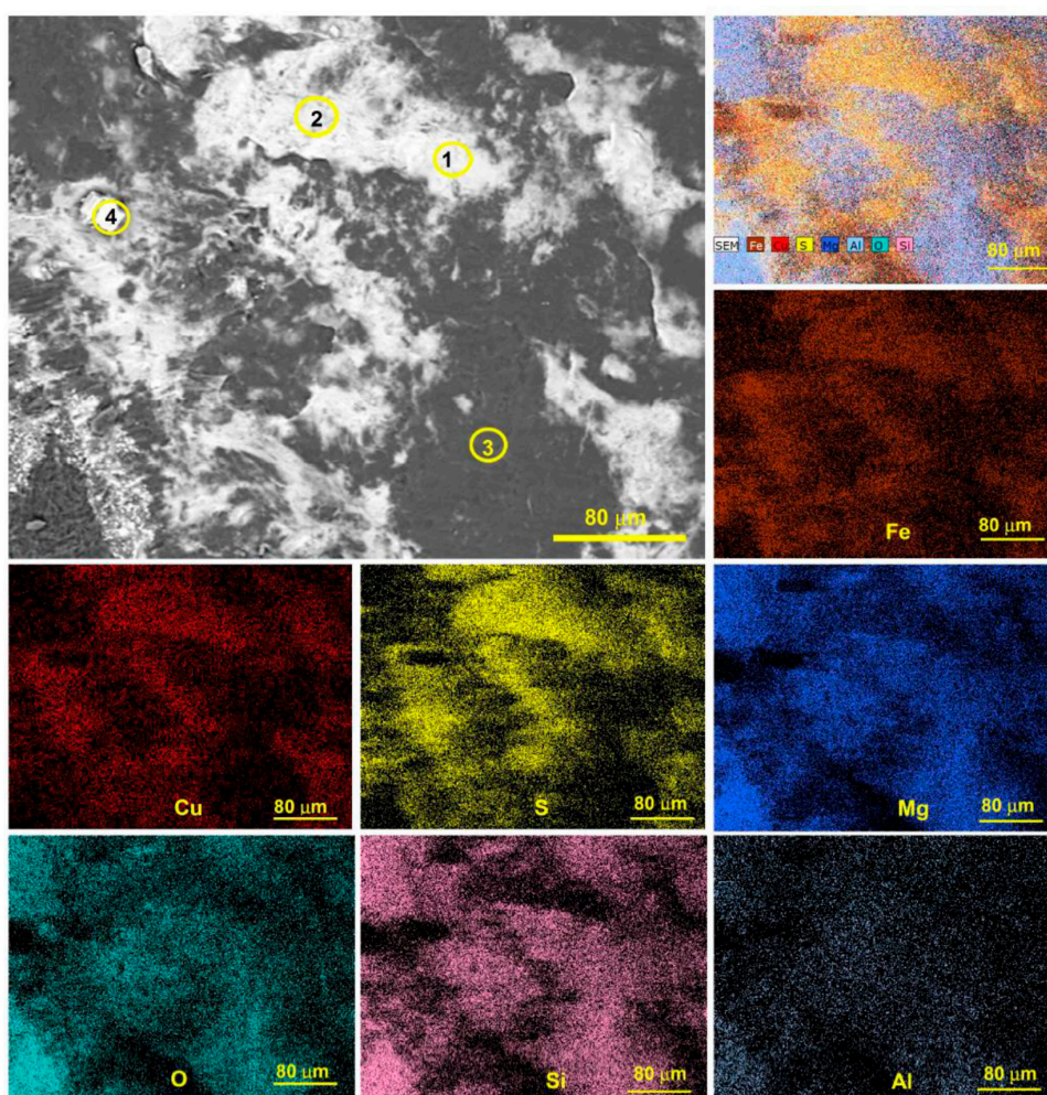
Fig. 2. Scanning microscopy image and elemental maps of natural growth surface of a typical valleriite-containing rock sample from Kingash deposit. Numbers in SEM image designate spots whose composition is presented in Table 1
