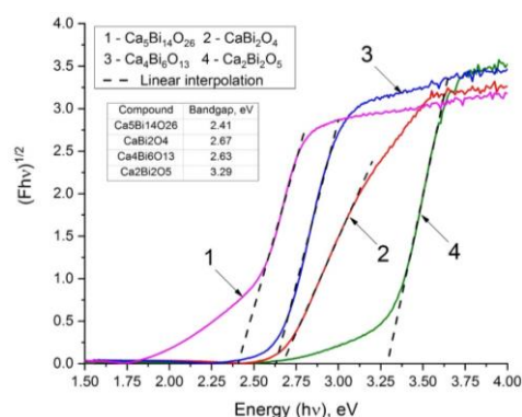
Figure 2. Tauc plots for all the as-synthesized calcium bismuthate samples for indirect transitions.
