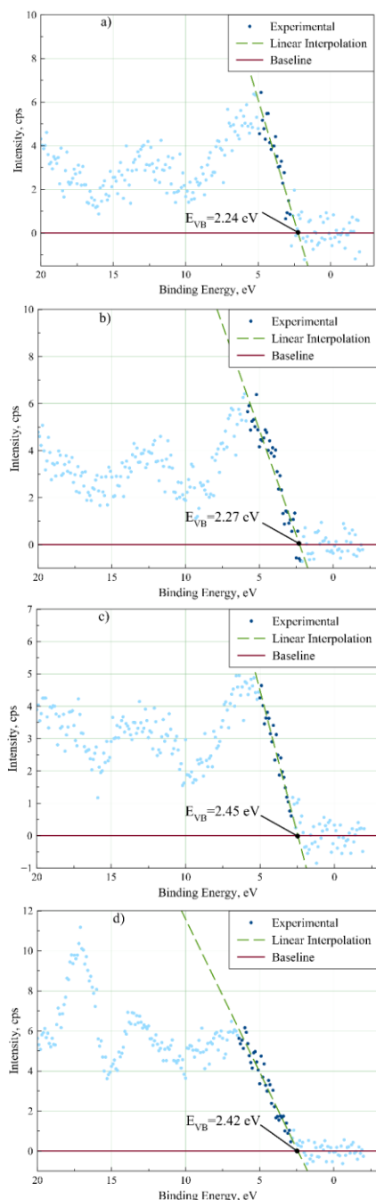
Figure 3. XPS spectra of the O 2p bands for the calcium bismuthates: (a) \text{Ca}_5\text{Bi}_{14}\text{O}_{26} , (b) \text{CaBi}_2\text{O}_4 , (c) \text{Ca}_4\text{Bi}_6\text{O}_{13} , and (d) \text{Ca}_2\text{Bi}_2\text{O}_5 .
