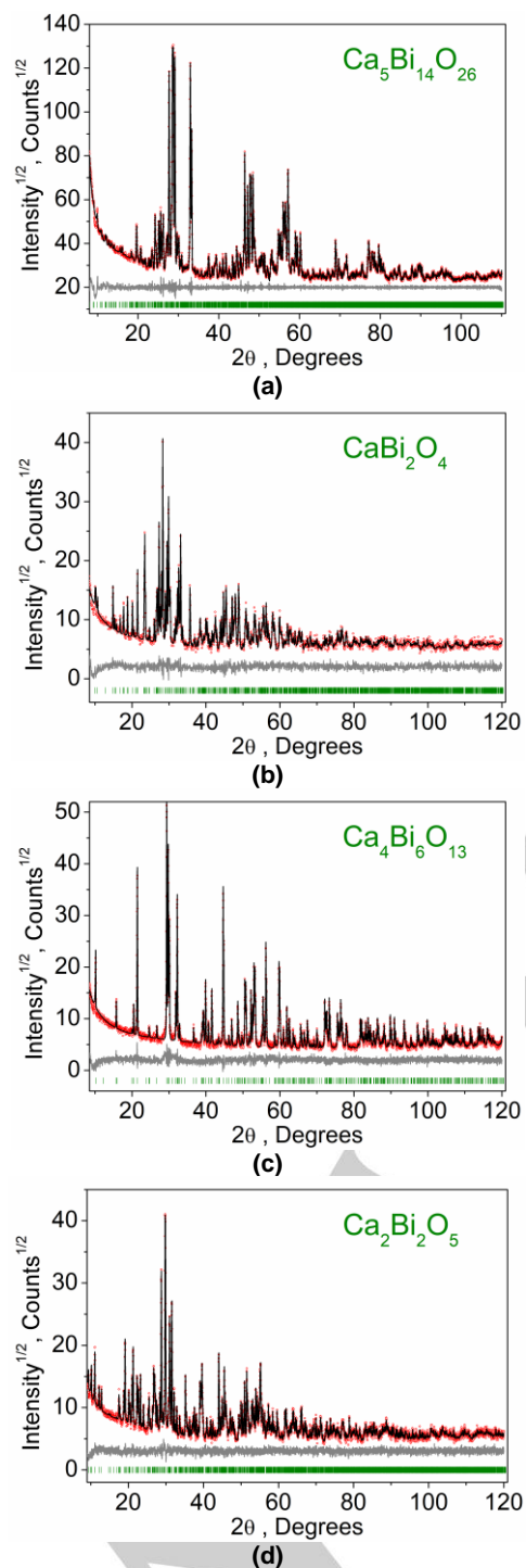
7 8 9 10 11 12 13 14 15 16 17 18 19 20 21 22 23 24 25 26 27 28 29 30 31 32 33 34 35 36 37 38 39 40 41 42 43 44 45 46 47 48 49 50 51 52 53 54 55 56 57 58 59 60 61 62 63 64 65 Figure 1. Difference Rietveld plots of the as-prepared calcium bismuthates: (a) \text{Ca}_5\text{Bi}_{14}\text{O}_{26} , (b) \text{CaBi}_2\text{O}_4 , (c) \text{Ca}_4\text{Bi}_6\text{O}_{13} , and (d) \text{Ca}_2\text{Bi}_2\text{O}_5 .
