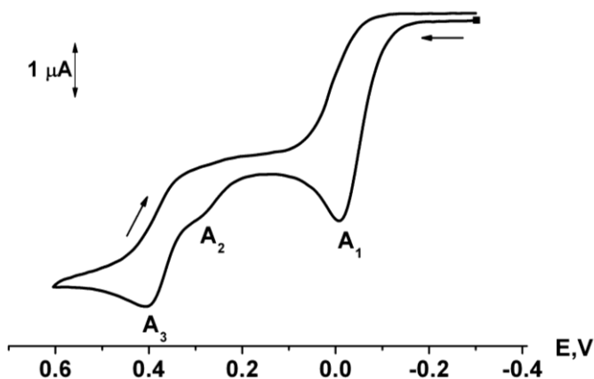
Fig. 3. The cyclic voltammogram of \text{Cp}(\text{CO})_2\text{RePt}(\mu\text{-C=CHPh})[\text{P}(\text{OEt})_3]_2 ( 2a ) at Pt-electrode in MeCN (0.1 M \text{Et}_4\text{NBF}_4 , C = 2 mM, scan rate 25 \text{mV s}^{-1} , potentials vs. \text{Ag}/0.1 M \text{AgNO}_3 in MeCN)
