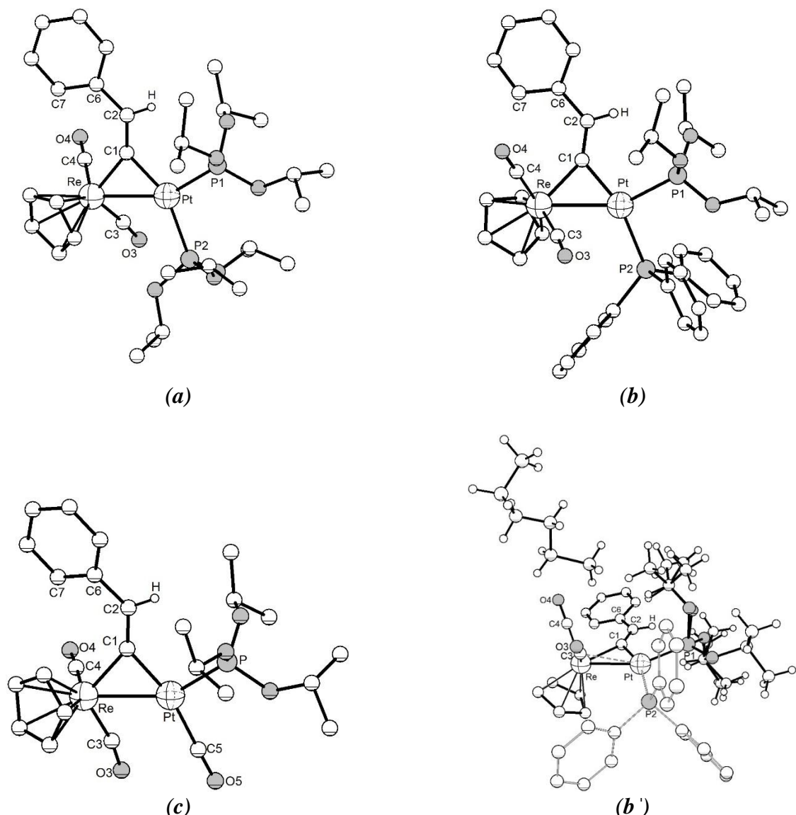
Fig. 1. Molecular structures of \text{Cp}(\text{CO})_2\text{RePt}(\mu\text{-C}=\text{CHPh})[\text{P}(\text{OPr}^i)_3]_2 ( 1a ) – (a); \text{Cp}(\text{CO})_2\text{RePt}(\mu\text{-C}=\text{CHPh})[\text{P}(\text{OPr}^i)_3](\text{PPh}_3) ( 1b ) – without (b) and with hexane molecule (b'); \text{Cp}(\text{CO})_2\text{RePt}(\mu\text{-C}=\text{CHPh})[\text{P}(\text{OPr}^i)_3](\text{CO}) ( 1c ) – (c). All hydrogen atoms in 1a-c except that of the phenylvinylidene ligand, of disorder \text{OPr}^i_3 -groups, and hexane in (b') are omitted for clarity.
