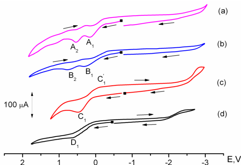
Fig. 2. The cyclic voltammograms of complexes: (a) – \text{Cp}(\text{CO})_2\text{RePt}(\mu\text{-C=CHPh})[\text{P}(\text{OEt})_3]_2 ( 2a ), (b) – \text{Cp}(\text{CO})_2\text{RePt}(\mu\text{-C=CHPh})[\text{P}(\text{OEt})_3](\text{PPh}_3)_2 ( 2b ), (c) – \text{Cp}(\text{CO})_2\text{RePt}(\mu\text{-C=CHPh})[\text{P}(\text{OEt})_3](\text{CO}) ( 2c ), (d) – \text{Cp}(\text{CO})_2\text{Re=C=CHPh} , at GC-electrode in MeCN (0.1 M \text{Et}_4\text{NBF}_4 , C = 2 mM, scan rate 25 \text{ mV s}^{-1} , potentials vs. Ag/0.1 M \text{AgNO}_3 in MeCN)
