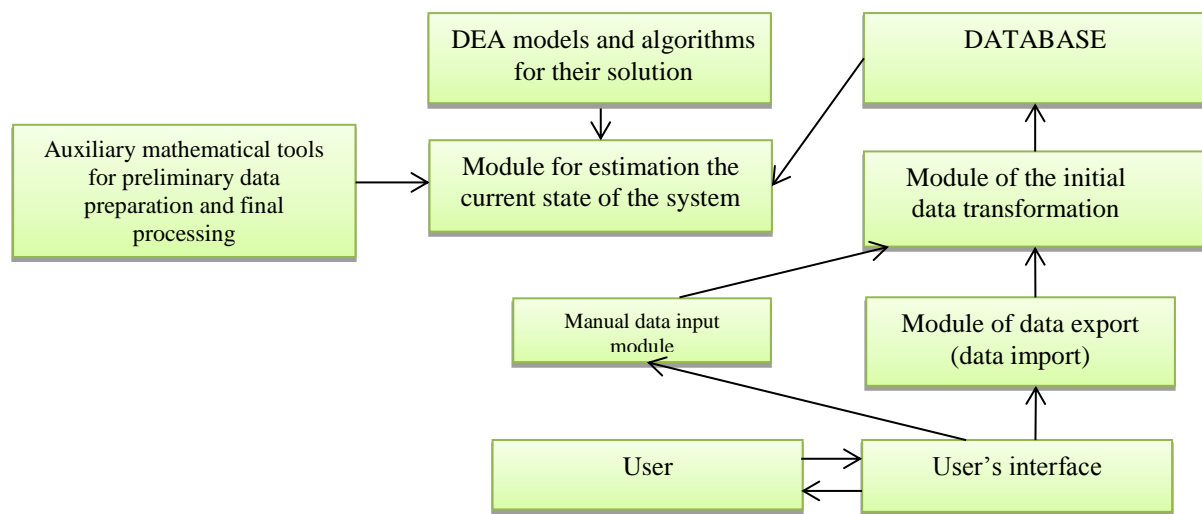
Figure 2. DEA.Block diagram of the DSS using the DEA method
