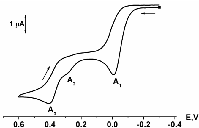
Fig. 3. The cyclic voltammogram of \text{Cp}(\text{CO})_2\text{RePt}(\mu\text{-C=CHPh})[\text{P}(\text{OEt})_3]_2 ( 2a ) at Pt-electrode in MeCN (0.1 M \text{Et}_4\text{NBF}_4 , C = 2 \text{ mM} , scan rate 25 \text{ mV s}^{-1} , potentials vs. Ag/0.1 M \text{AgNO}_3 in MeCN)
