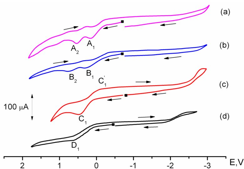
Fig. 2. The cyclic voltammograms of complexes: (a) – \text{Cp}(\text{CO})_2\text{RePt}(\mu\text{-C=CHPh})[\text{P}(\text{OEt})_3]_2 ( 2a ), (b) – \text{Cp}(\text{CO})_2\text{RePt}(\mu\text{-C=CHPh})[\text{P}(\text{OEt})_3](\text{PPh}_3)_2 ( 2b ), (c) – \text{Cp}(\text{CO})_2\text{RePt}(\mu\text{-C=CHPh})[\text{P}(\text{OEt})_3](\text{CO}) ( 2c ), (d) – \text{Cp}(\text{CO})_2\text{Re=C=CHPh} , at GC-electrode in MeCN (0.1 M \text{Et}_4\text{NBF}_4 , C = 2 \text{ mM} , scan rate 25 \text{ mV s}^{-1} , potentials vs. Ag/0.1 M \text{AgNO}_3 in MeCN)
