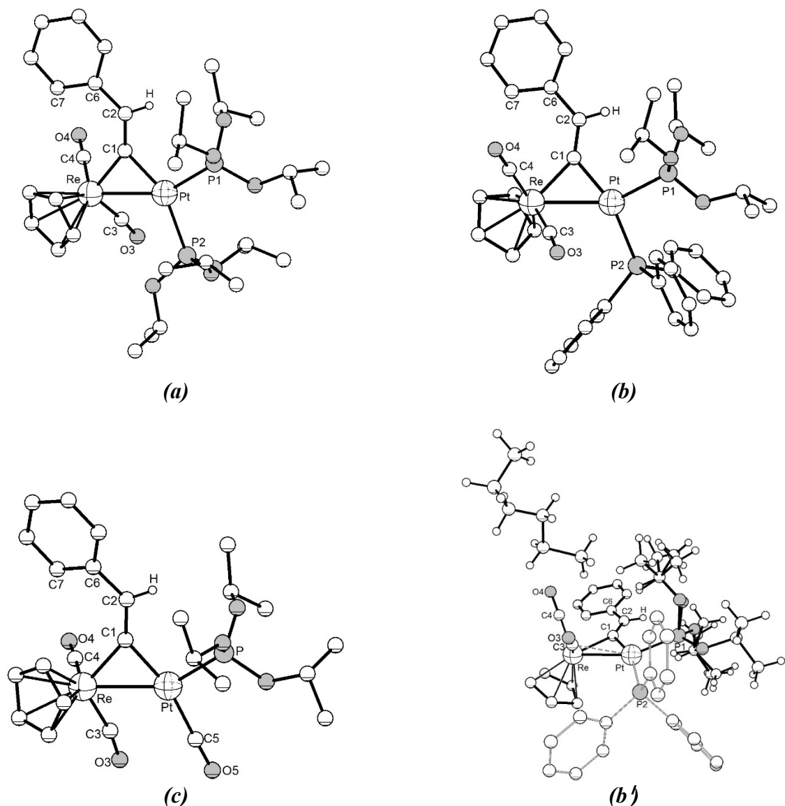
Fig. 1. Molecular structures of \text{Cp}(\text{CO})_2\text{RePt}(\mu\text{-C}=\text{CHPh})[\text{P}(\text{OPr}^i)_3]_2 ( 1a ) – (a); \text{Cp}(\text{CO})_2\text{RePt}(\mu\text{-C}=\text{CHPh})[\text{P}(\text{OPr}^i)_3](\text{PPh}_3) ( 1b ) – without (b) and with hexane molecule (b'); \text{Cp}(\text{CO})_2\text{RePt}(\mu\text{-C}=\text{CHPh})[\text{P}(\text{OPr}^i)_3](\text{CO}) ( 1c ) – (c). All hydrogen atoms in 1a-c except that of the phenylvinylidene ligand, of disorder \text{OPr}^i_3 -groups, and hexane in (b) are omitted for clarity.
