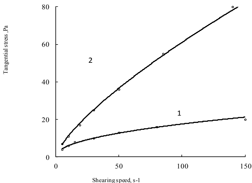
Fig. 1. The CWS flow rheogram: 1 – Cs = 40.5 %, 2 – Cs = 37 %
