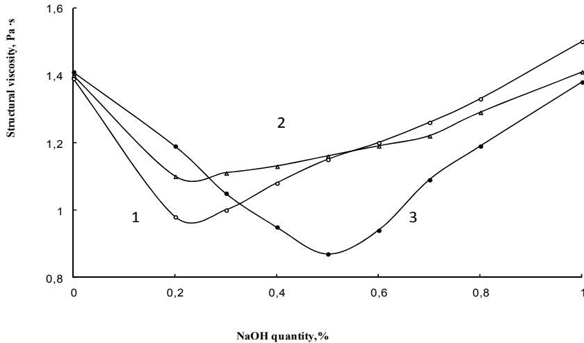
Fig. 2. Plot CWS structural viscosity against putting natrium hydroxide quantity (Cs – 46 %). (Coal ash content 1 – 4.6; 2 – 5.3; 3 – 7.6 %)
