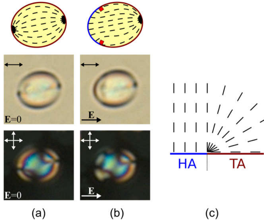
Fig. 2. POM images of 5CB nematic droplet doped with anionic surfactant HOBBDDA in the weight ratio 5CB : HOBBDDA = 1 : 0.014 in the initial state (a) and under DC electric field of 0.07 \text{ V}/\mu\text{m} directed from left to right (b). Photos are taken with switched-off analyzer (middle row) and in crossed polarizers (bottom row). The droplet's sizes along the major and minor axes are 10 and 8 \mu\text{m} , respectively. The director configurations in the central section of the droplet are presented at the top row. A scheme of cross-section of the splay-type ring defect dividing the areas with homeotropic (HA) and tangential (TA) surface anchoring (c). Hereinafter, the polarizer orientation is indicated by the double arrows. The direction of electric field \mathbf{E} is shown by the single arrow.
