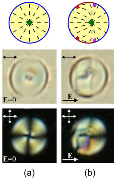
Fig. 4. POM images of 5CB nematic droplet doped with a mixture of the anionic surfactant HOBDDA and cationic surfactant CTAB with weight concentrations 1% and 0.5%, respectively, in initial state (a) and under DC electric field of 0.07 \text{ V}/\mu\text{m} directed from left to right (b). Photos are taken with switched-off analyzer (middle row) and in crossed polarizers (bottom row). The droplet size is 10 \mu\text{m} . The director configurations in central section of droplet are presented at the top row.
