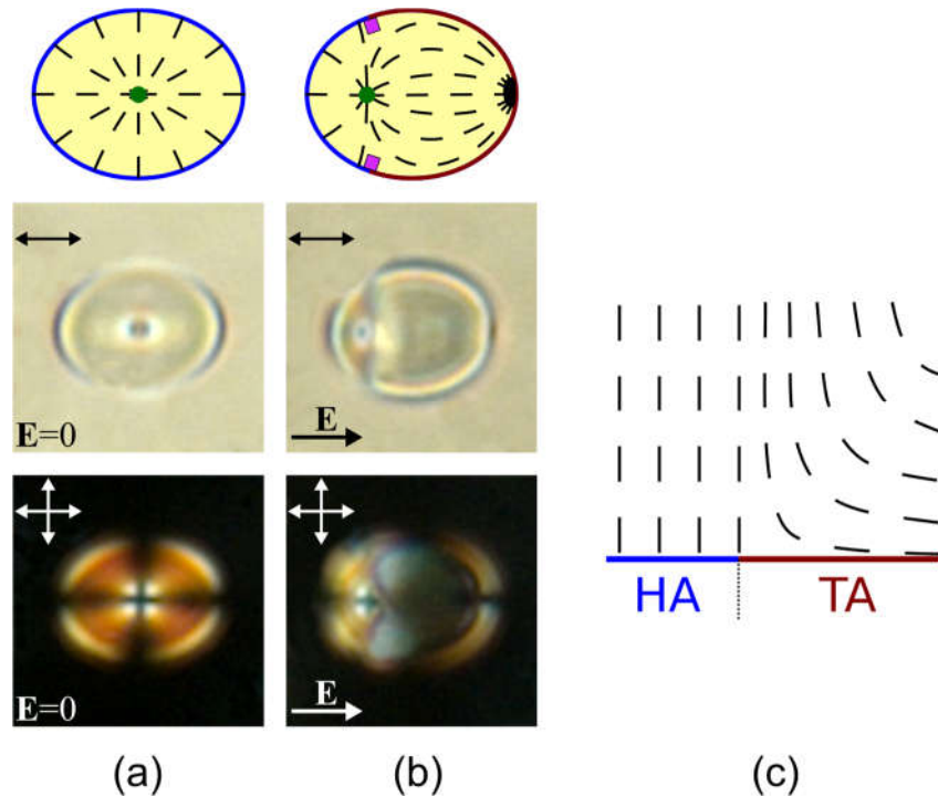
Fig. 3. POM images of 5CB nematic droplet doped with anionic surfactant HOBBDDA in the weight ratio 5\text{CB} : \text{HOBBDDA} = 1 : 0.017 in the initial state (a) and under DC electric field of 0.09 \text{ V}/\mu\text{m} directed from left to right (b). Photos are taken with switched-off analyzer (middle row) and in crossed polarizers (bottom row). The droplet's sizes along the major and minor axes are 12 and 9 \mu\text{m} , respectively. The director configurations in the central section of droplet are presented at the top row. The cross-section of bend-type ring defect dividing the areas with homeotropic (HA) and tangential (TA) surface anchoring (c).
