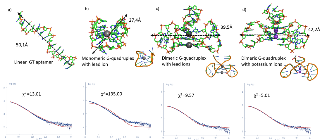
Fig. 3. 3D models of GT aptamer. Comparison of the SAXS model from experiment (blue dashed curve) with structures of GT aptamer (red curve) obtained with MD simulations for Solution No.1. a) linear shape of GT aptamer, b) monomeric quadruplex with \text{Pb}^{2+} ion, c) dimeric quadruplex with \text{Pb}^{2+} ions, d) dimeric quadruplex with potassium ions. Carbon atoms are shown in green, nitrogen in blue, phosphorus in orange, oxygen in red, \text{Pb}^{2+} ions are presented as grey balls, and potassium ions are purple balls. Linear dimensions of the complexes are given in angstroms. Hydrogen atoms are not shown in the figure
