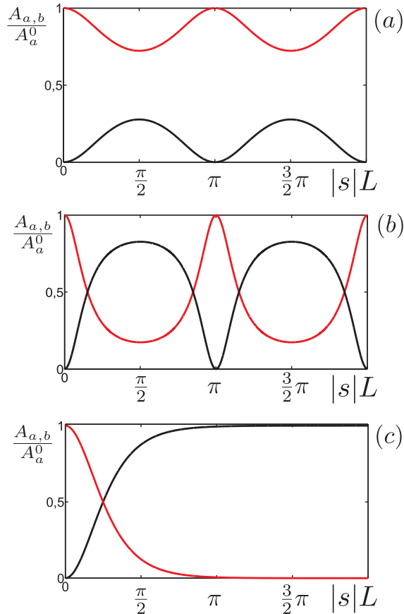
FIG. 2: Dynamics of the normalized over A_0 = |\alpha|^2 quantum field's amplitude as a function of the dimensionless parameter |s|L where s is given in Eq.13 and L is the interaction length. The red line is the function A_a/A_a^0 and the black one is the A_b/A_a^0 . a) P = 10 b) P = 1.1 c) P = 0.4
