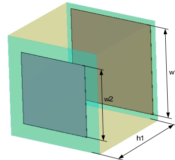
Figure 1. Unit cell
