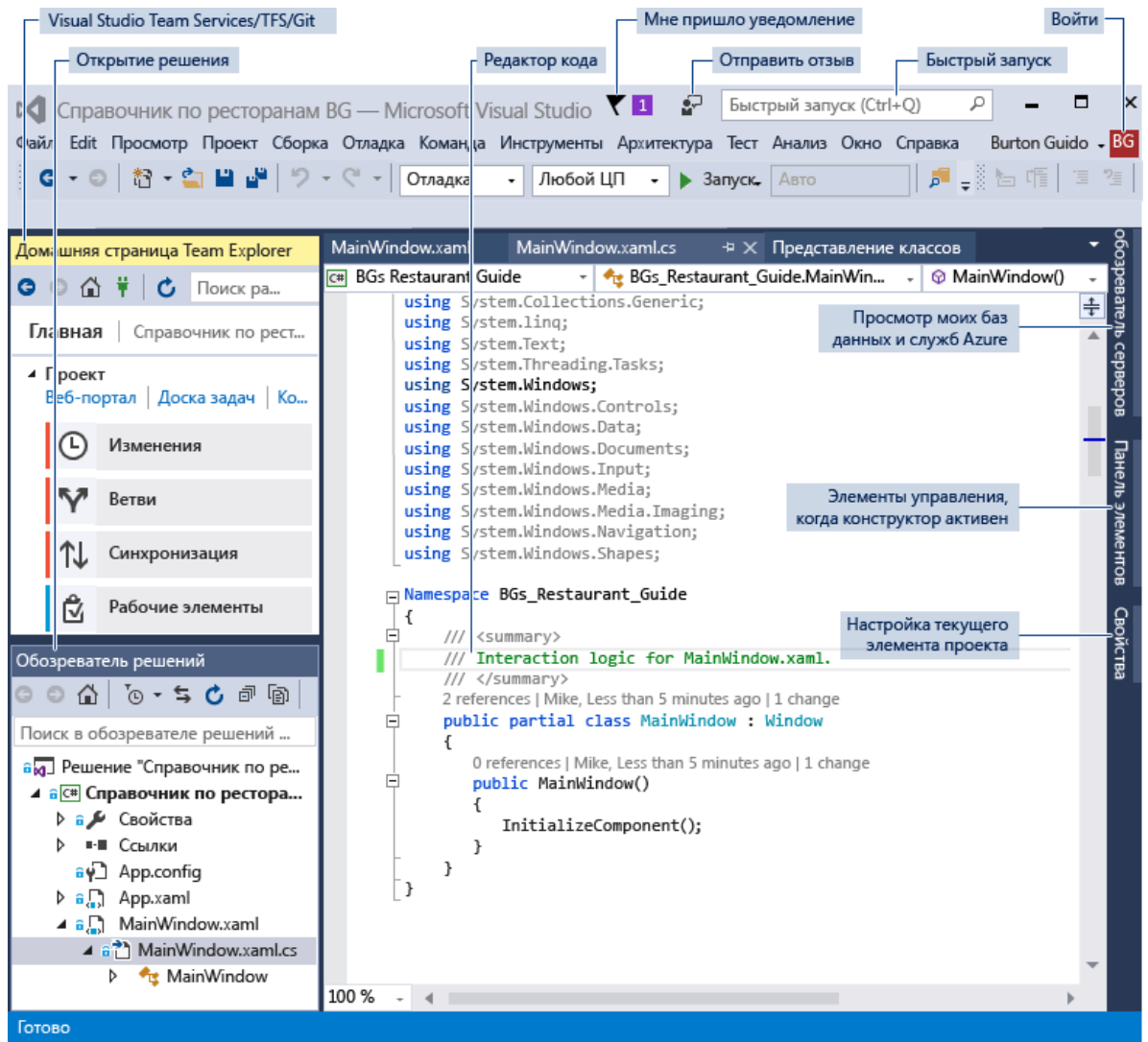
6 " 7 " " Visual Studio
