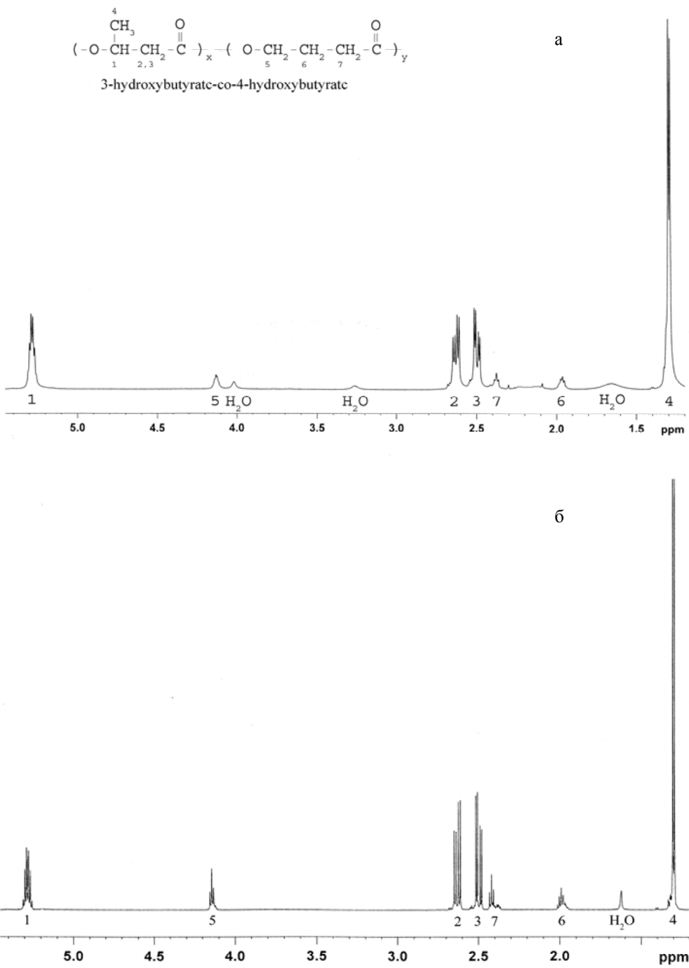
Fig. 2. 1 H-NMR spectrum of the P(3HB-co-4HB) with content of 4HB 8.7 mol % (a) and 16 mol % (b)
