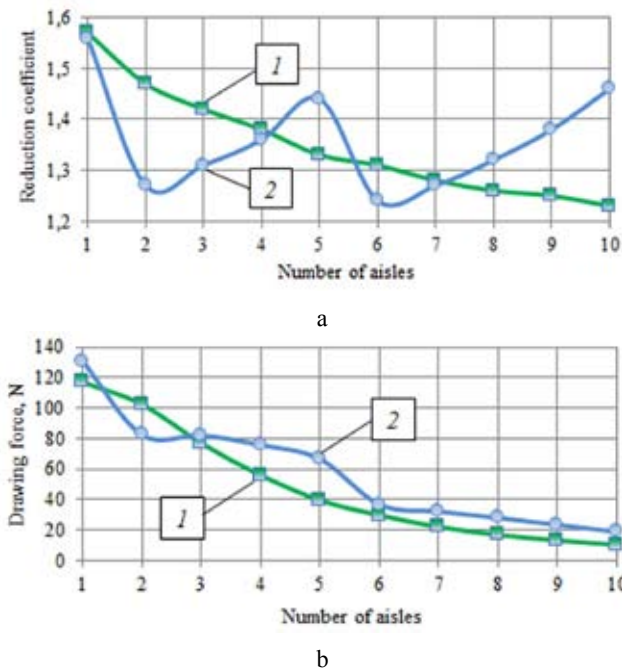
Fig. 6. Changing of unit reduction (a) and force of drawing (b) the aisles for the proposed (1) and existing (2) processing routes for new 925 standard silver alloy
