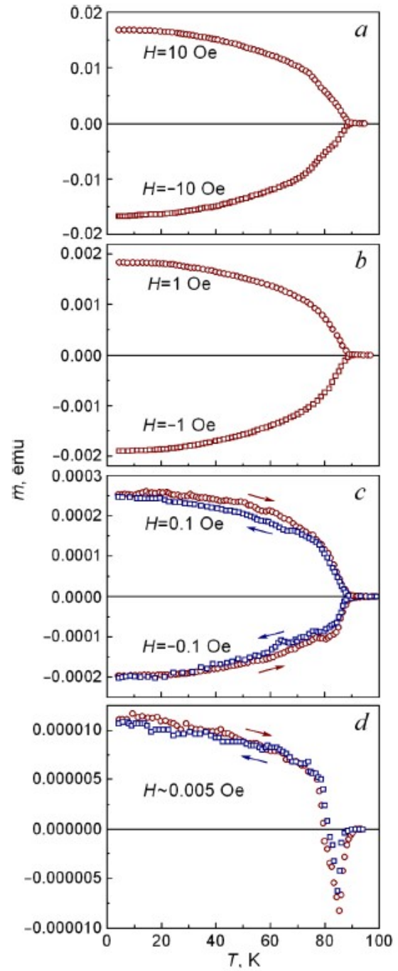
Figure 4. Temperature dependences of \text{Cu}_2\text{MnBO}_5 magnetic moment measured in a magnetic field of \pm 10 Oe (a); \pm 1 Oe (b); \pm 0.1 Oe (c); \sim 0.005 Oe (d), directed along the crystallographic a axis. Sample weight is 14.4 mg.
