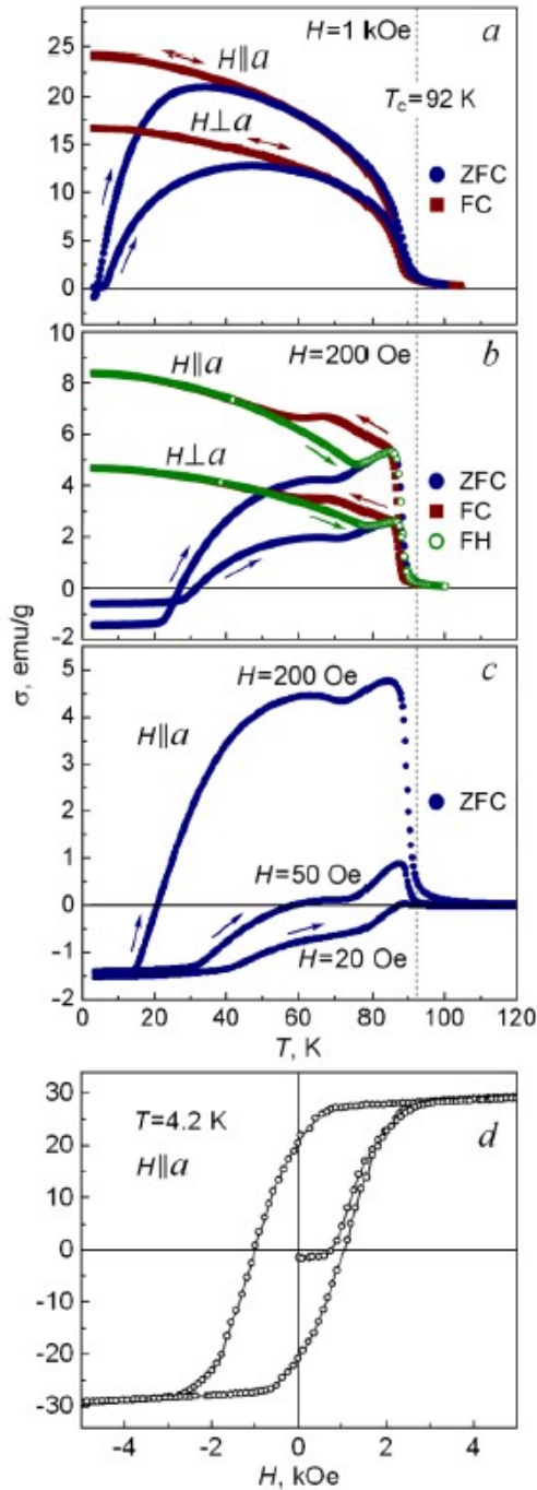
Figure 3. Temperature dependences of \text{Cu}_2\text{MnBO}_5 magnetization measured in a magnetic field of 1 kOe (a); 200 Oe (b); in ZFC mode (c). Magnetic hysteresis loop (d).
