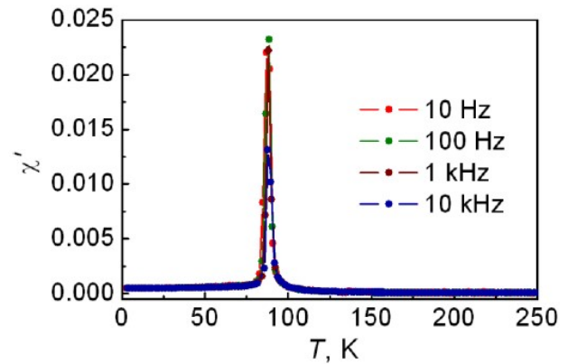
Figure 2. Temperature dependences of Cu 2 MnBO 5 AC magnetic susceptibility.
