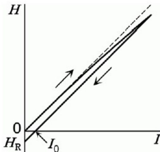
Figure 5. The dependence of the magnetic field of a superconducting solenoid from the electric current flowing through the coil.
