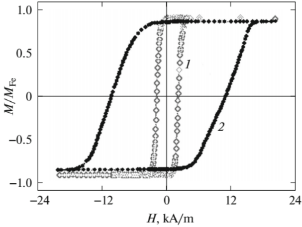
Fig. 1. Magnetic hysteresis loops of (1) Fe/Bi and (2) Bi/Fe two-layer films measured at T = 300 K.
