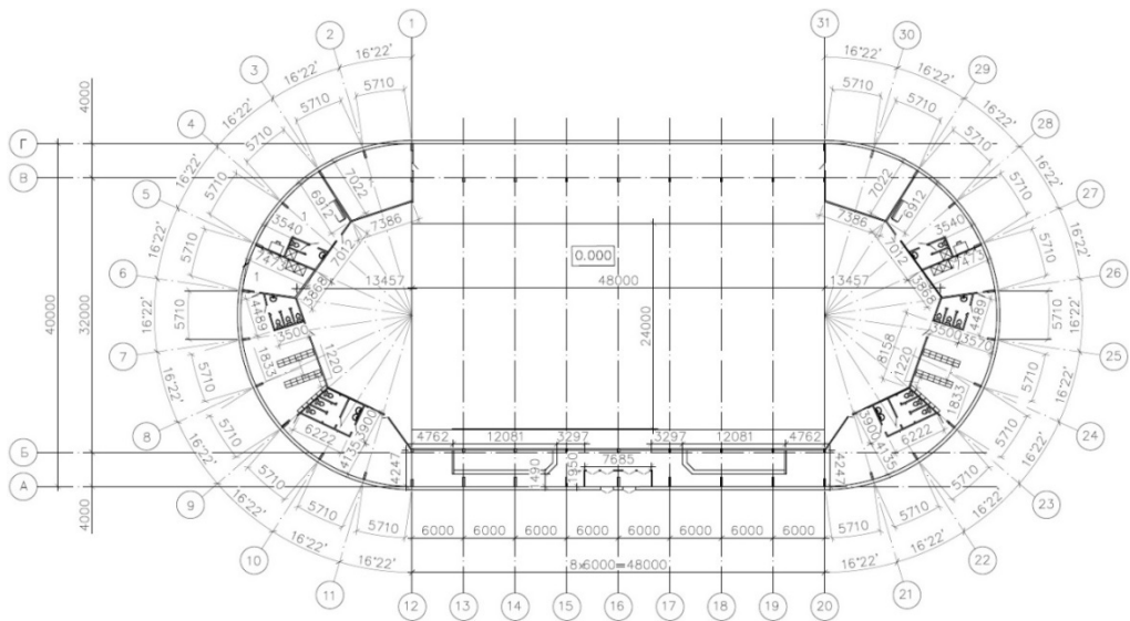
Fig. 2. Plan at + 0.000
