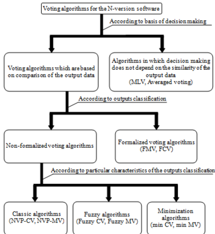
Figure 1. Classification of voting algorithms in N-version software.
