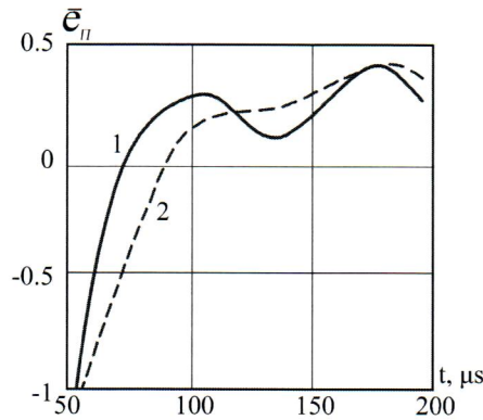
Fig. 7. Function of the impulse response vs ground electrical conductivity. Where \sigma = 2 S/m , 2 is \sigma_2 = 1.1 S/m
