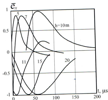
Fig. 2. Time-response characteristic of the two-layer medium reaction for the EE_X/MR_Y system \sigma_1 = 1 S/m, \sigma_2 = 0.1 S/m, \tau_u = 50 \mu s, t = 100 \mu s
