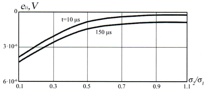
Fig. 4. Functional relation of signal amplitude vs electrical conductivity of the soil. Where h = 10 m , \sigma_1 = 1 S/m , \tau_u = 50 \mu s
