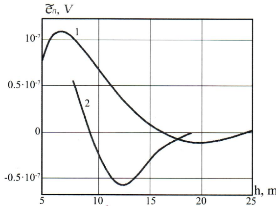
Fig. 3. Function of SI ( \tilde{e}_n ) vs the distance from the soil h . Here 1 is the EE_X/MR_Y system, 2 is the ME_X/MR_Y system, \sigma_1 = 1 S/m , \sigma_2 = 0.1 S/m , \tau_u = 50 \mu s , t = 100 \mu s
