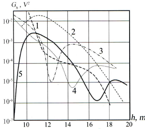
Fig. 5. Functional relation of the SI random component vs distance to the soil at the fixed time delay. Where 1 is t = 0 \mu s , 2 is t = 50 \mu s , 3 is t = 100 \mu s , 4 is t = 150 \mu s , 5 is t = 200 \mu s , \sigma_1 = 2 S/m , \sigma_2 = 0.1 S/m , \tau_u = 50 \mu s
