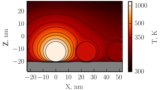
Figure 6: The temperature T distribution at t = 1 ns for first three OPW nanoparticles at the central cross-section, y = 0 . The n = 1 nanoparticle is exposed to pulsed laser radiation with I = 1.57 \times 10^8 \text{ W/cm}^2 intensity. Note that colormap is given in nonlinear scale for convenience.
