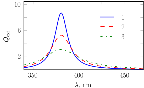
Figure 2: Extinction spectra of single Ag nanoparticle with R = 8 nm for different values of temperatures and states of matter: 1 — at room temperature; 2 — at the melting temperature in solid state; 3 — at the melting temperature in liquid state.
