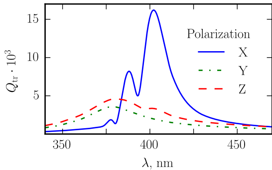
Figure 3: Transmission spectra of the OPW for different polarizations of laser radiation. Temperature of the system is T = 300 K.
