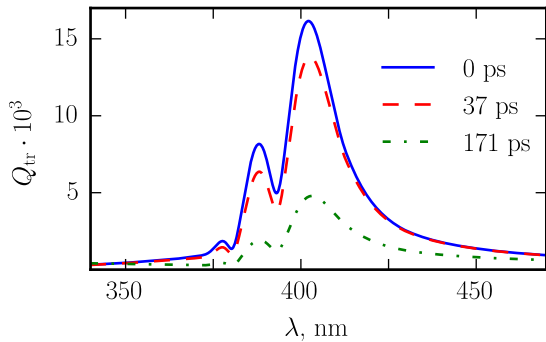
Figure 5: Transmission spectra of the OPW exposed to laser radiation with intensity I = 1.57 \times 10^8 \text{ W/cm}^2 at different moments of time: the initial moment of time, t = 0 (solid line); the beginning of n = 1 nanoparticle melting, t = 37 ps (dashed line); the end of n = 1 nanoparticle melting, t = 171 ps (dash-dot line).
