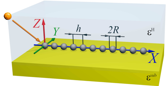
Figure 1: Schematic illustration of the of OPW geometry used in numerical simulations.
