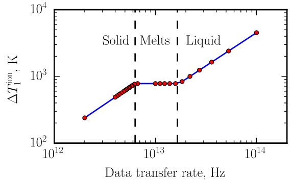
Figure 7: The temperature change of ionic subsystem for n = 1 nanoparticle temperature change for different values of data transfer rate.
