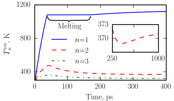
Figure 4: Temperature of ion subsystem for first, second and third OPW nanoparticles during 1 ns excitation with \lambda = 402 nm and intensity I = 1.57 \times 10^8 W/cm 2 . The inset shows the slow increase of T_2^{\text{ion}} in 250–1000 ps time range.
