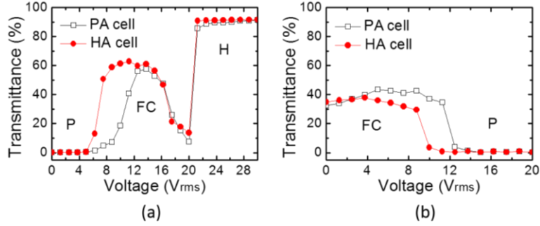
Fig. 3. Voltage-dependent transmittance at operation frequencies of (a) 1 kHz and (b) 100 kHz in cell R of 4.0 \pm 0.5 \mu\text{m} cell gap.
